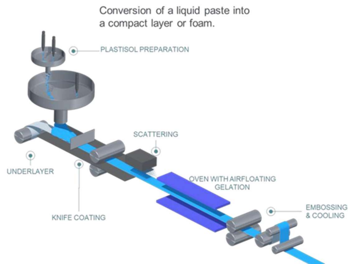
Figure 4: Coating process
