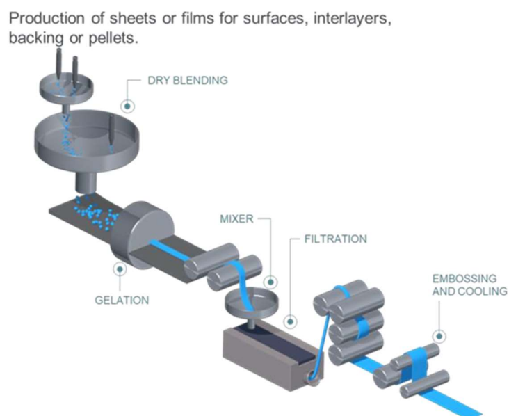
Figure 5: Calendering process
